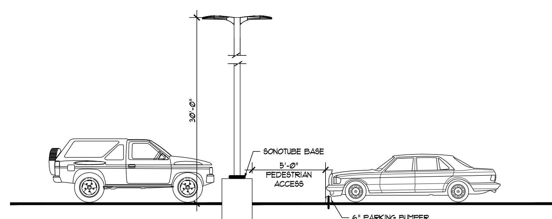
3 TYP. PEDESTRIAL ACCESS DETAIL FOR ILLUMINATING A PARKING AREA SCALE: NTS PLUMBING/MECHANICAL/LED LOT LMS
