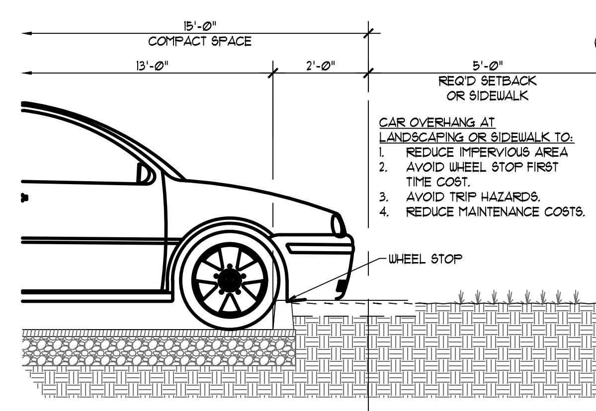
4 CAR OVERHANG AT LANDSCAPING OR SIDEWALK SCALE: 1/2" = 1'-0"
