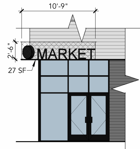
SOUTH ELEVATION
