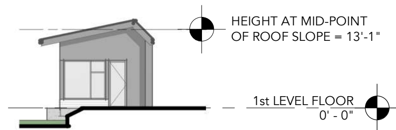
3 OFFICE - NORTH ELEVATION SCALE: 1/16" = 1'-0"
