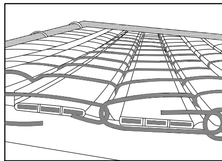
TYPICAL SLAT KNUCKLED SELVAGES DETAIL
