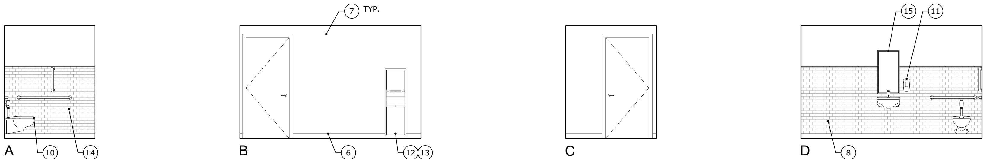
2 BATHROOM 107 - INTERIOR ELEVATIONS SCALE: 1/4" = 1'-0"
