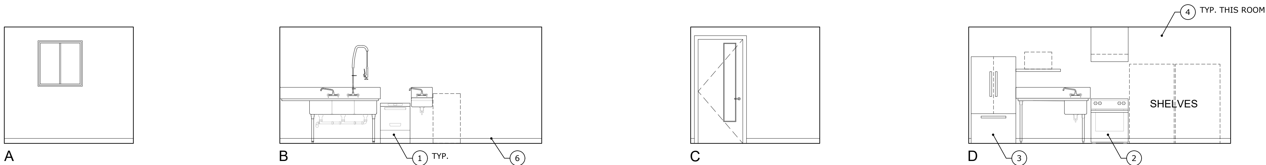
1 WARMING KITCHEN 106 - INTERIOR ELEVATIONS SCALE: 1/4" = 1'-0"
