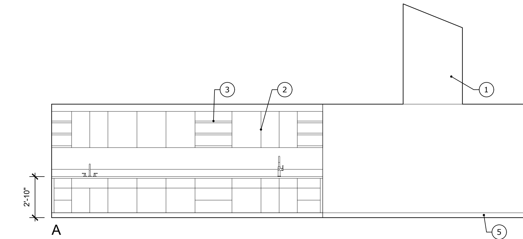
2 CLASSROOM 102 - INTERIOR ELEVATIONS SCALE: 1/4" = 1'-0"
