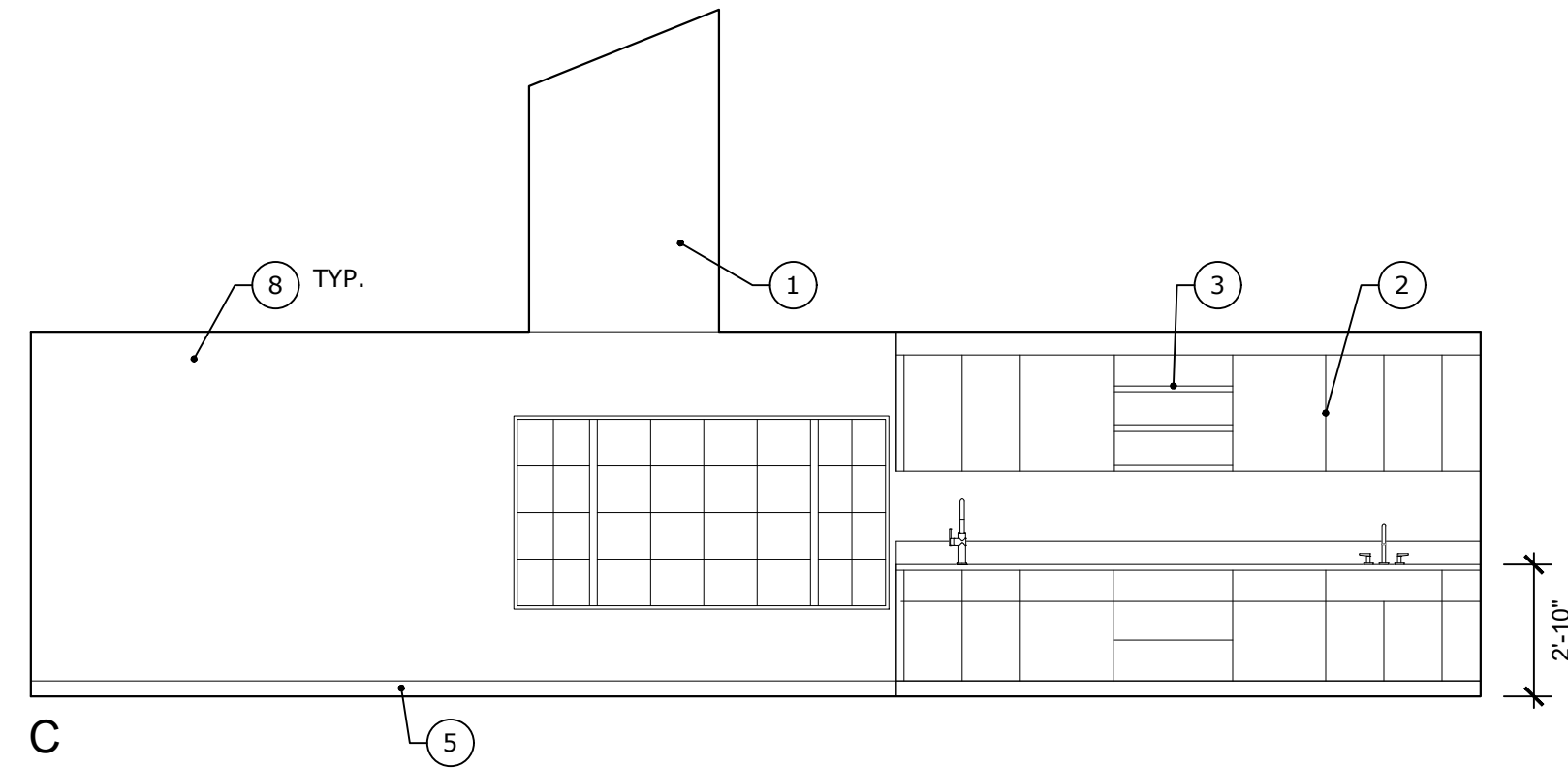
2 CLASSROOM 102 - INTERIOR ELEVATIONS SCALE: 1/4" = 1'-0"
