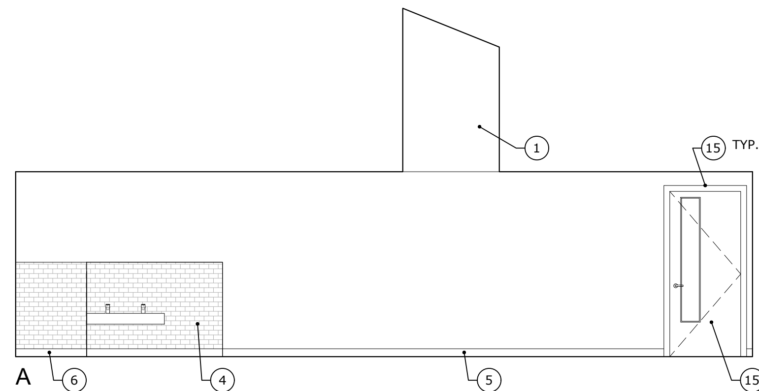
1 CLASSROOM 101 - INTERIOR ELEVATIONS SCALE: 1/4" = 1'-0"
