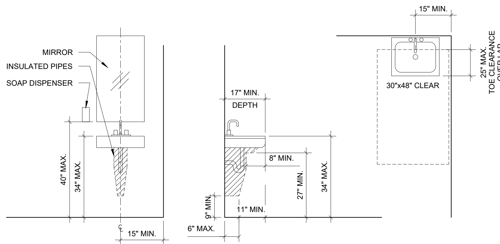
TYP. ADA BATHROOM LAVATORY
