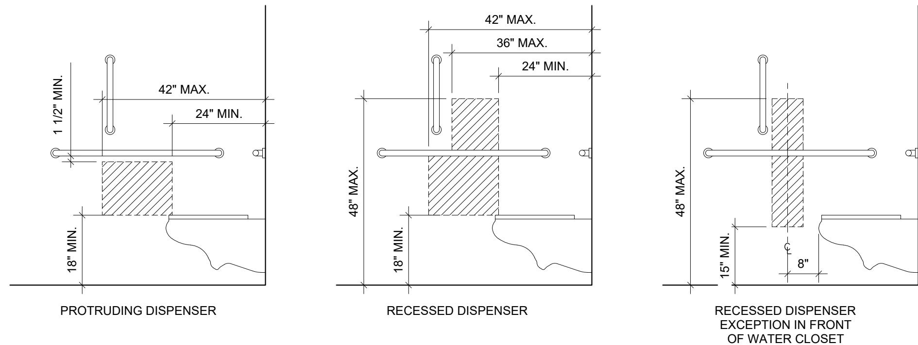
TYP. DISPENSER LOCATIONS NEAR GRAB BARS
