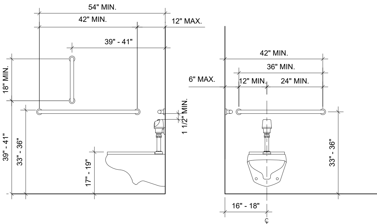
TYP. ADA WATER CLOSET AND GRAB BARS - ADULT
