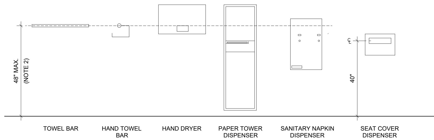
TOILET ROOM ACCESSORY MOUNTING HEIGHTS
