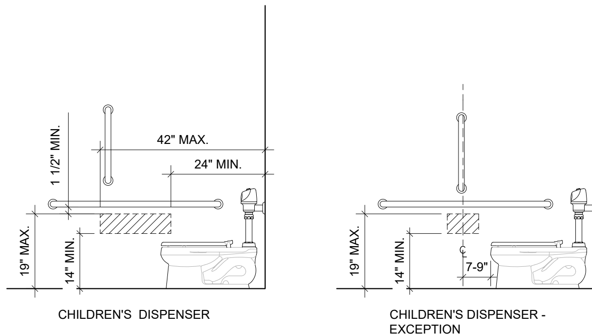
TYP. DISPENSER LOCATIONS NEAR GRAB BARS - CHILD HEIGHT
