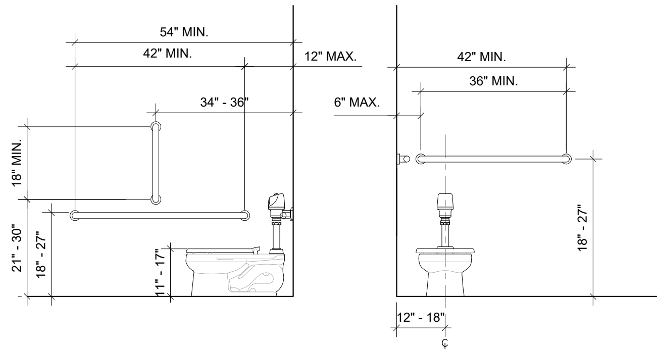
TYP. ADA WATER CLOSET AND GRAB BARS - CHILD HEIGHT
