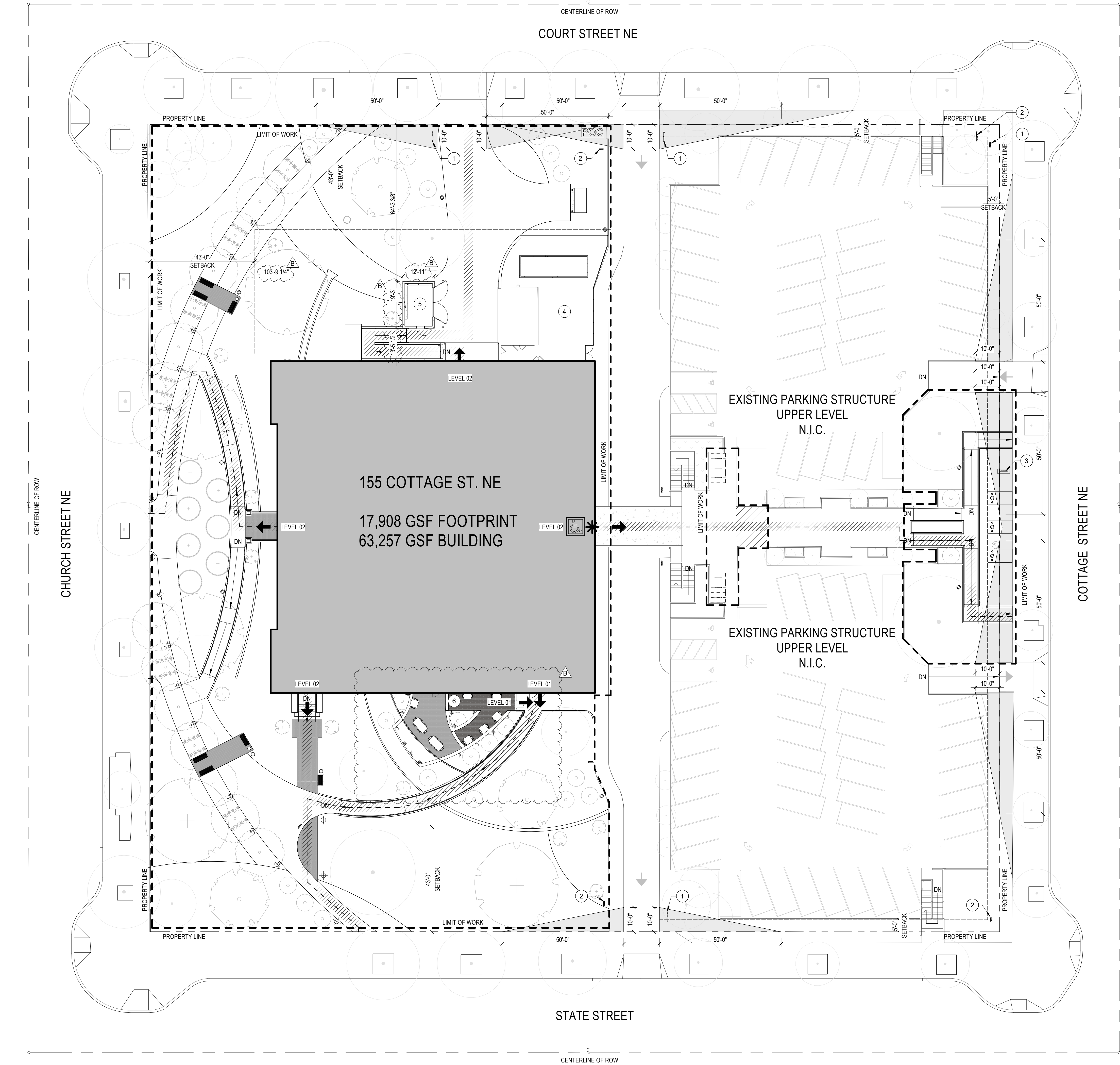
2 SITE OVERVIEW PLAN - LEVEL 02 1" = 20'-0"
