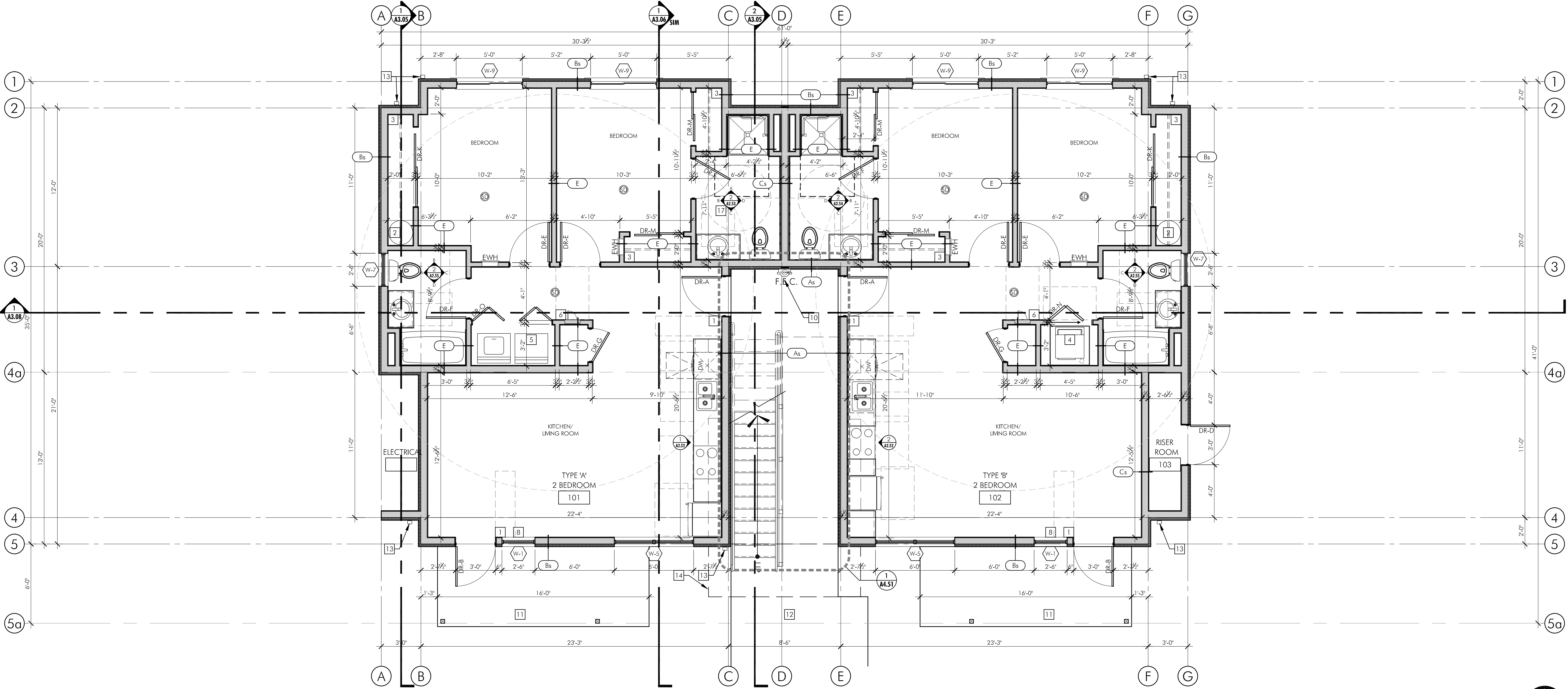
1 BUILDING TYPE 3 - LEVEL 01 FLOOR PLAN - ACCESSIBLE - BUILDING G
