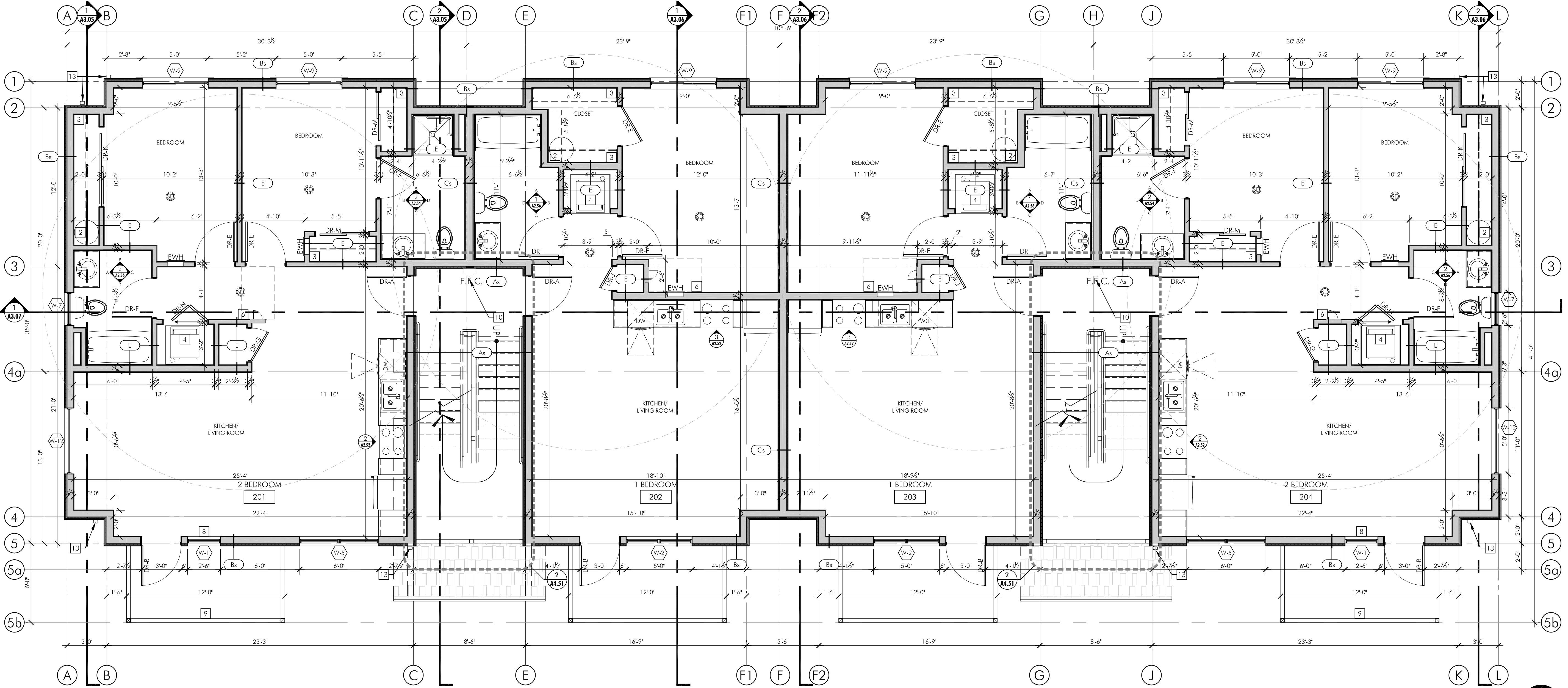
1 BUILDING TYPE 2 - LEVEL 02 FLOOR PLAN
