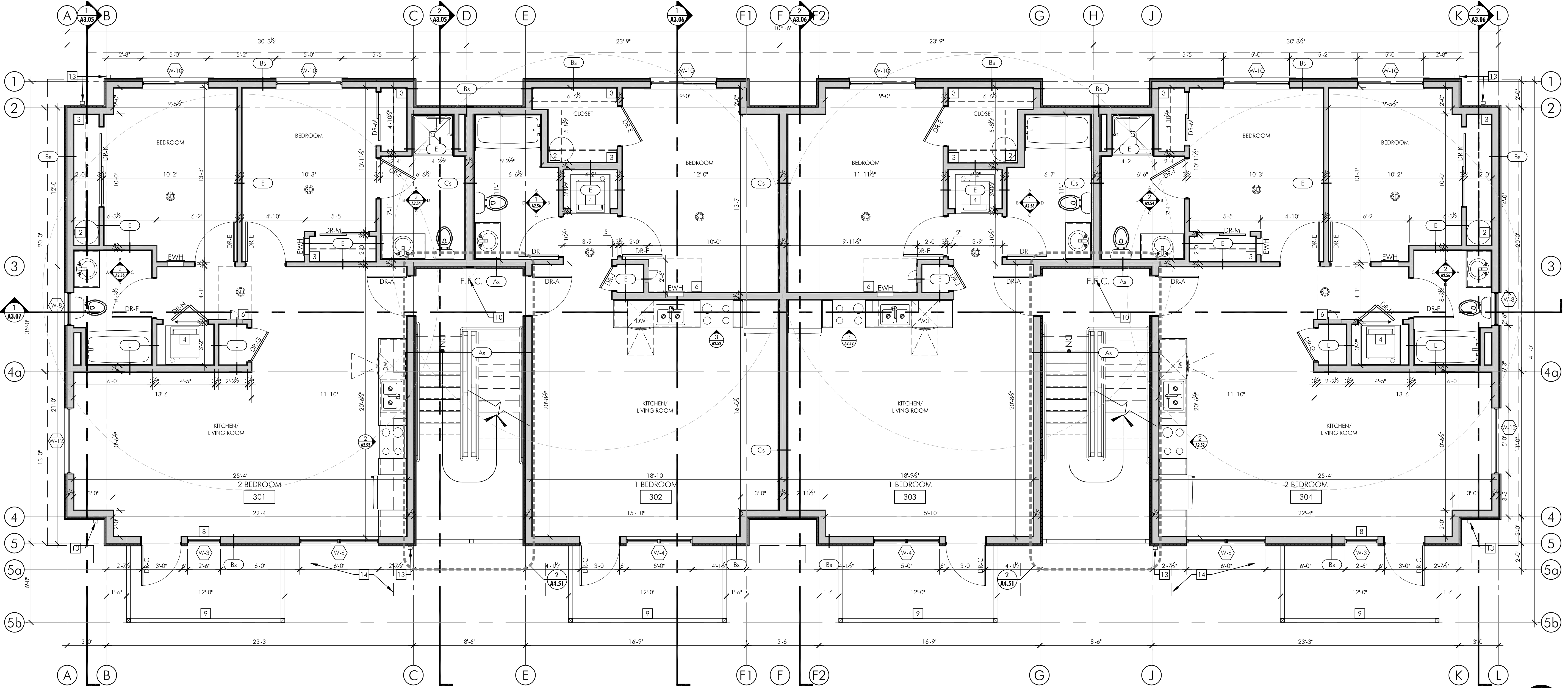
1 BUILDING TYPE 2 - LEVEL 03 FLOOR PLAN
