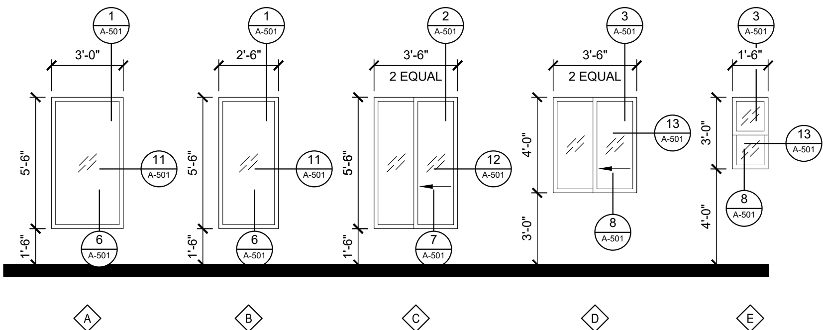
WINDOW ELEVATIONS
