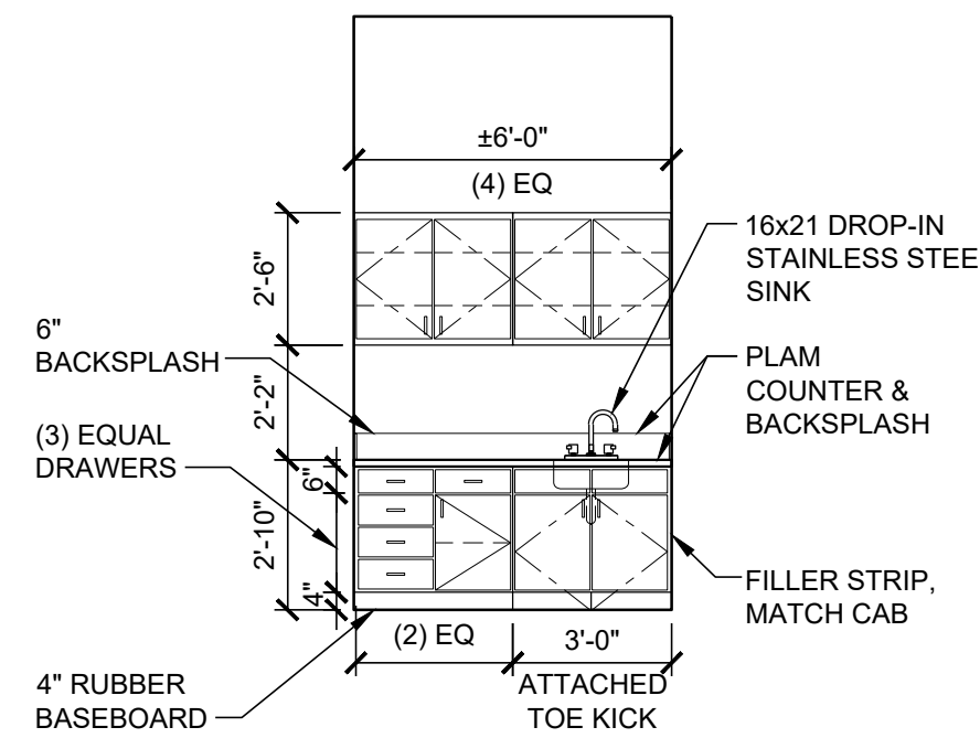
D CLASSROOM 2 - 202
