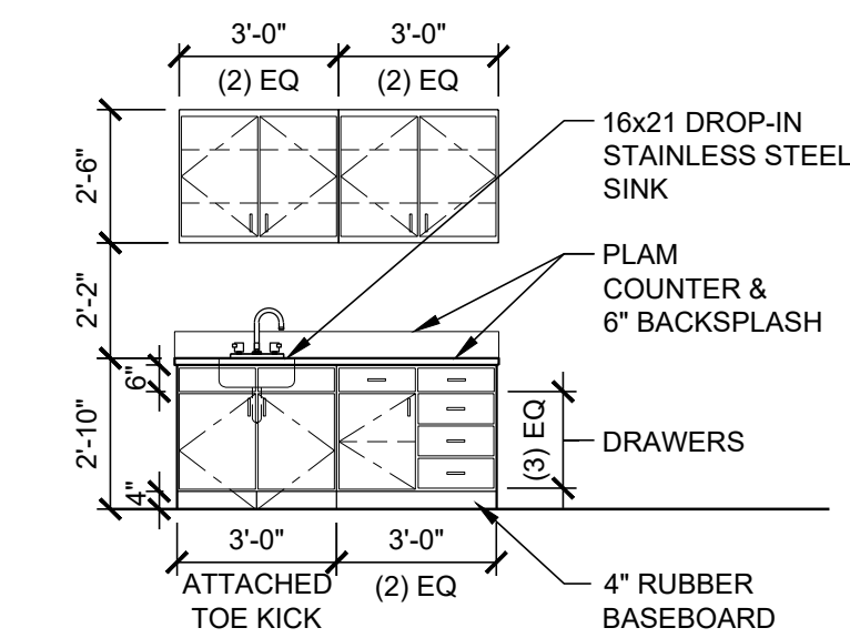
C CLASSROOM 1 - 201
