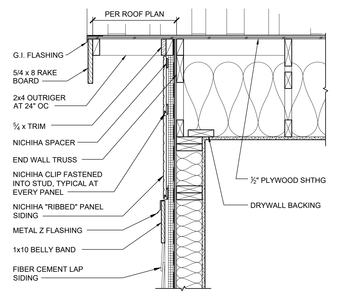
4 TYPICAL RAKE 1" = 1'-0"
