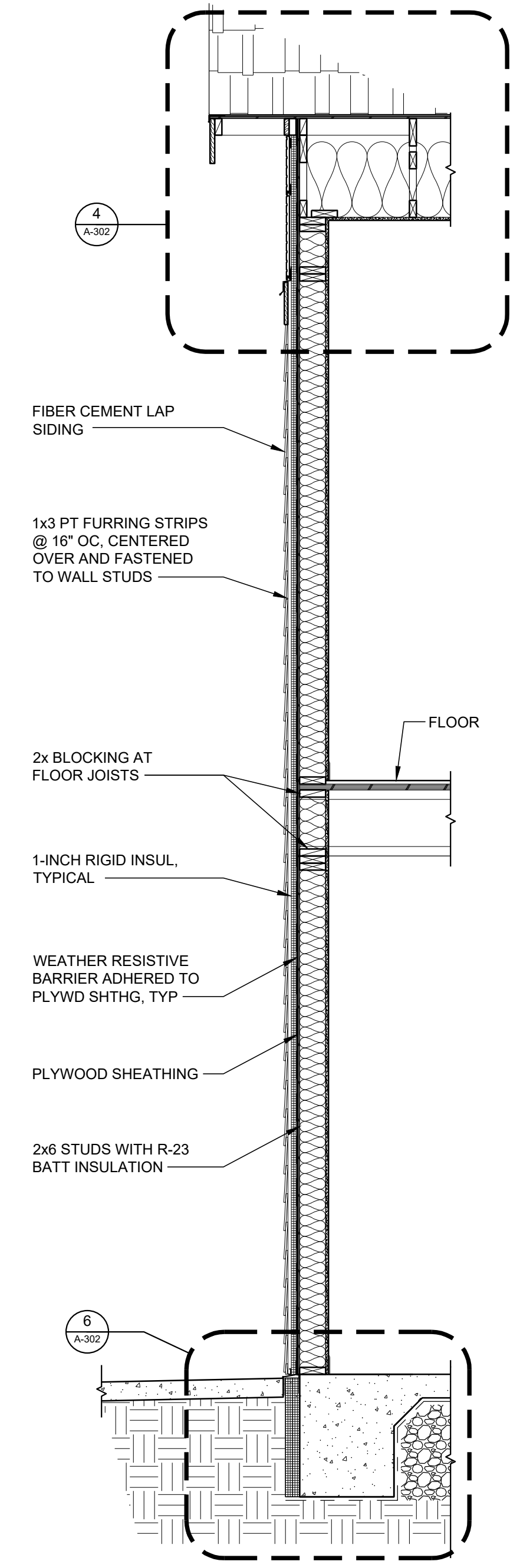
2 WALL SECTION - GABLE WALL 1/2" = 1'-0"
