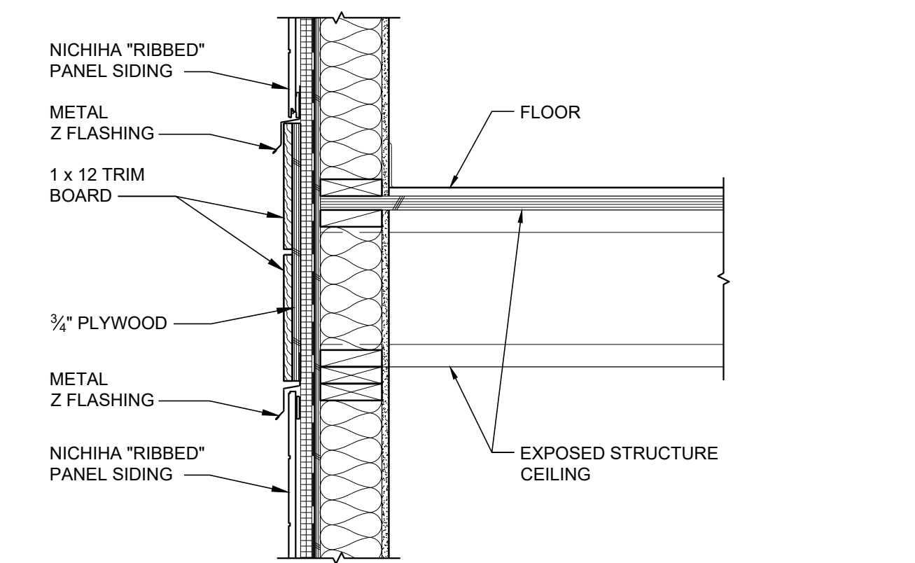
7 BELLY BAND TRIM 1" = 1'-0"
