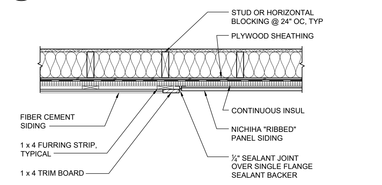
11 LAP SIDING TO NICHIHA PANEL 1" = 1'-0"
