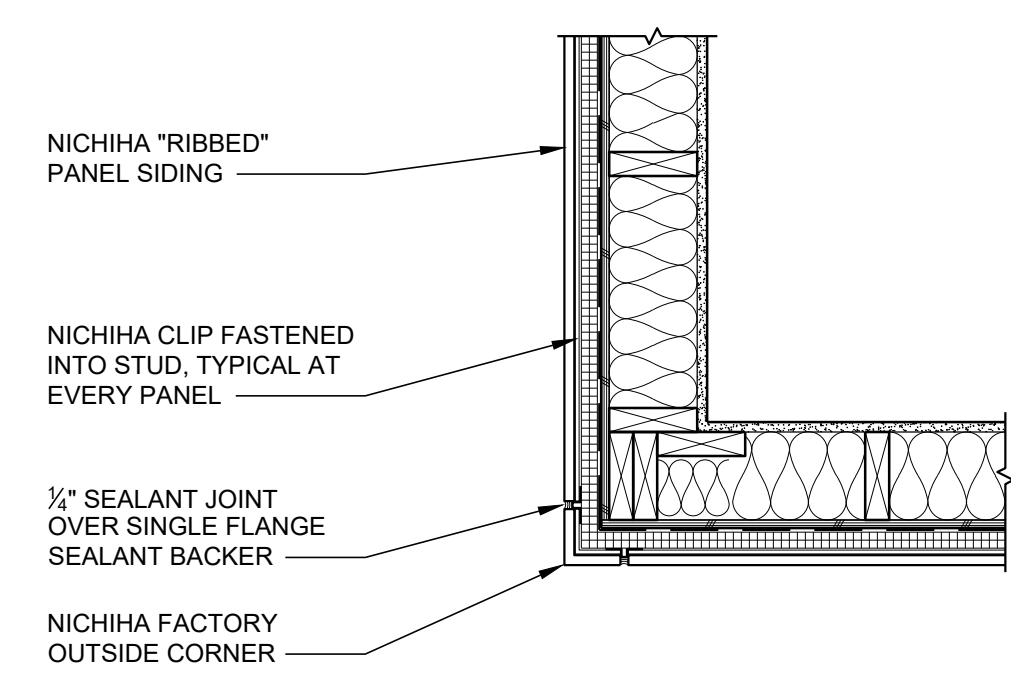
9 OUTSIDE CORNER AT NICHIHA SIDING 1" = 1'-0"
