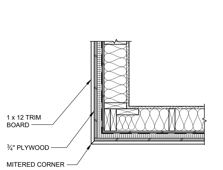
10 OUTSIDE CORNER AT SOFFIT 1" = 1'-0"
