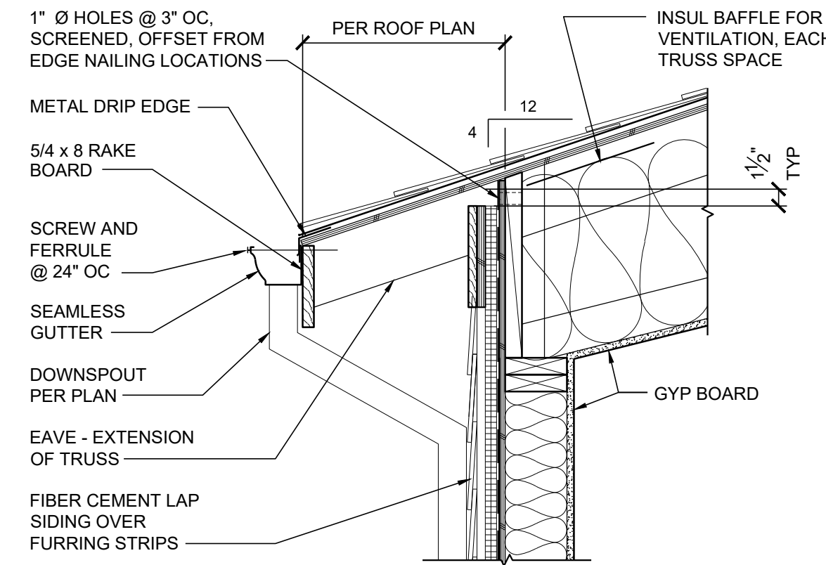
8 EAVE - NORTH 1" = 1'-0"
