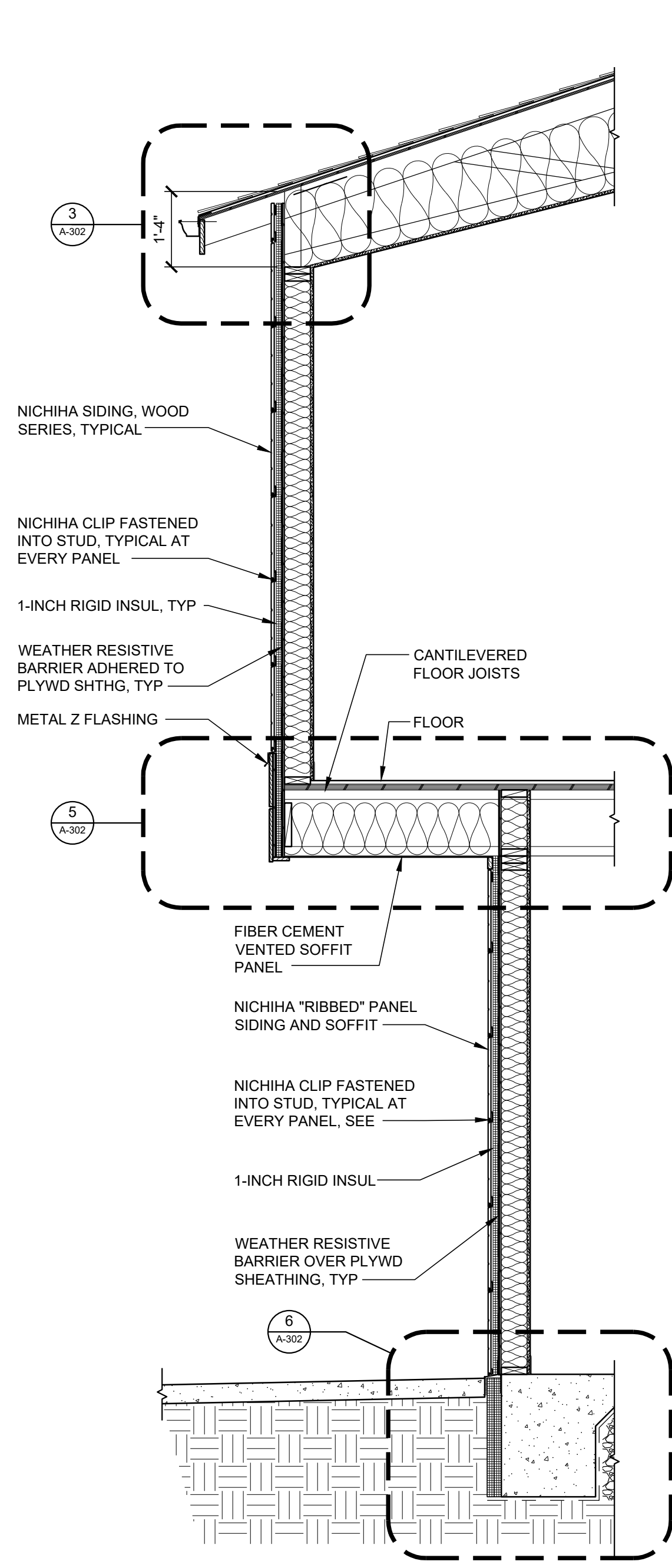
1 WALL SECTION - SOUTH WALL 1/2" = 1'-0"
