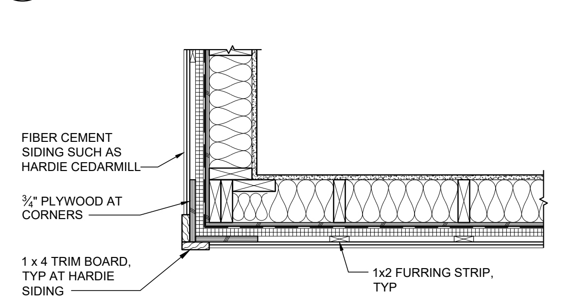
12 OUTSIDE CORNER AT LAP SIDING 1" = 1'-0"
