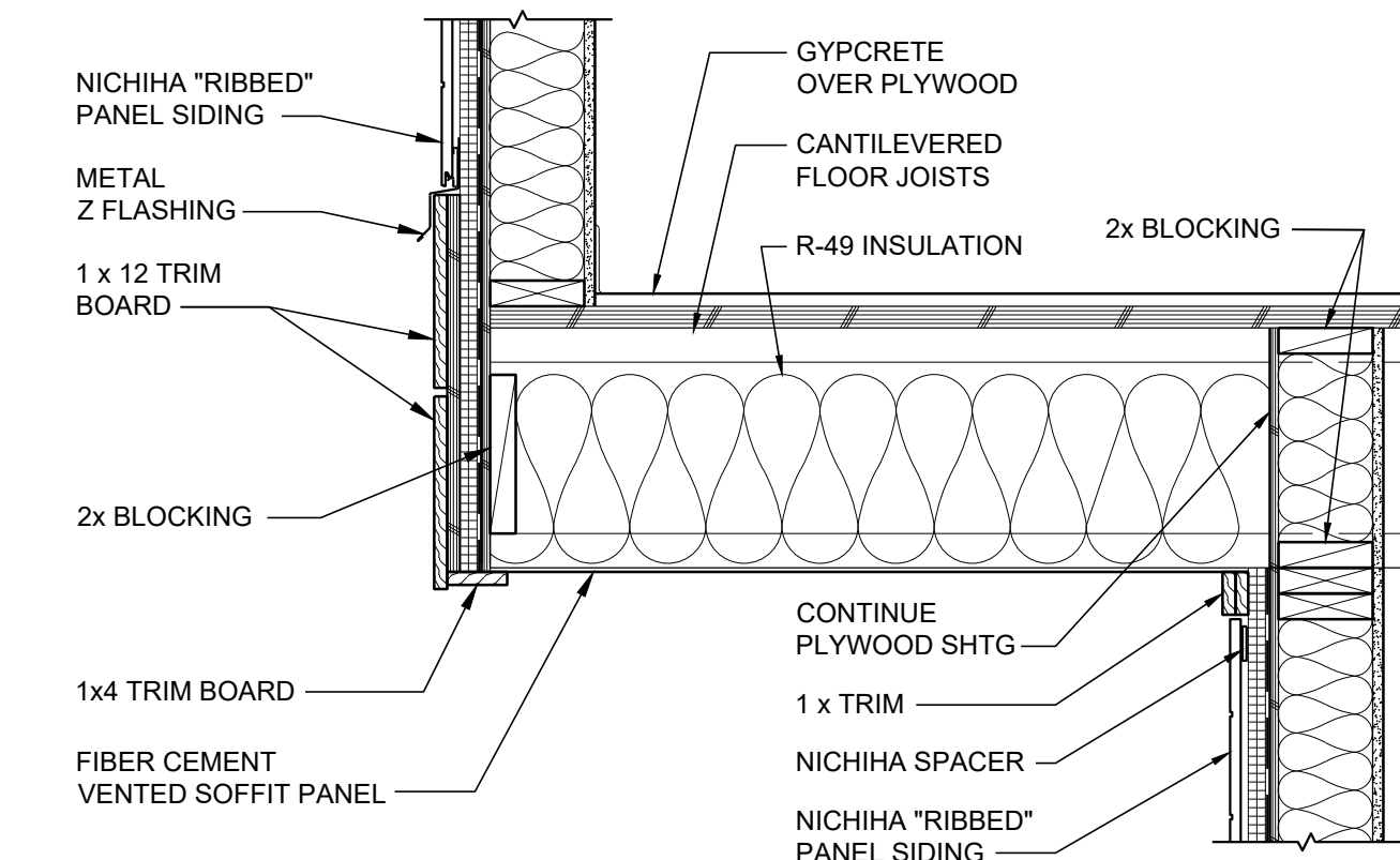
5 CANTILEVERED SOFFIT 1" = 1'-0"
