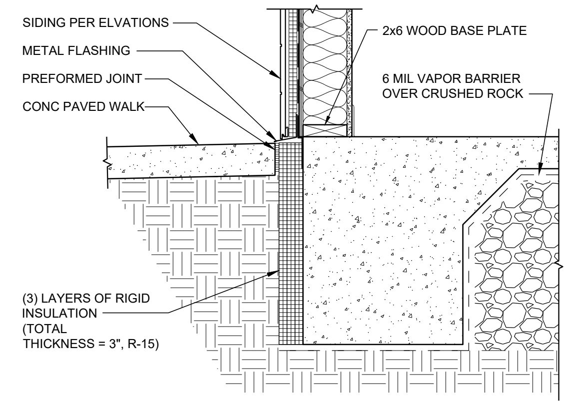
6 TYPICAL EXTERIOR WALL BASE 1" = 1'-0"
