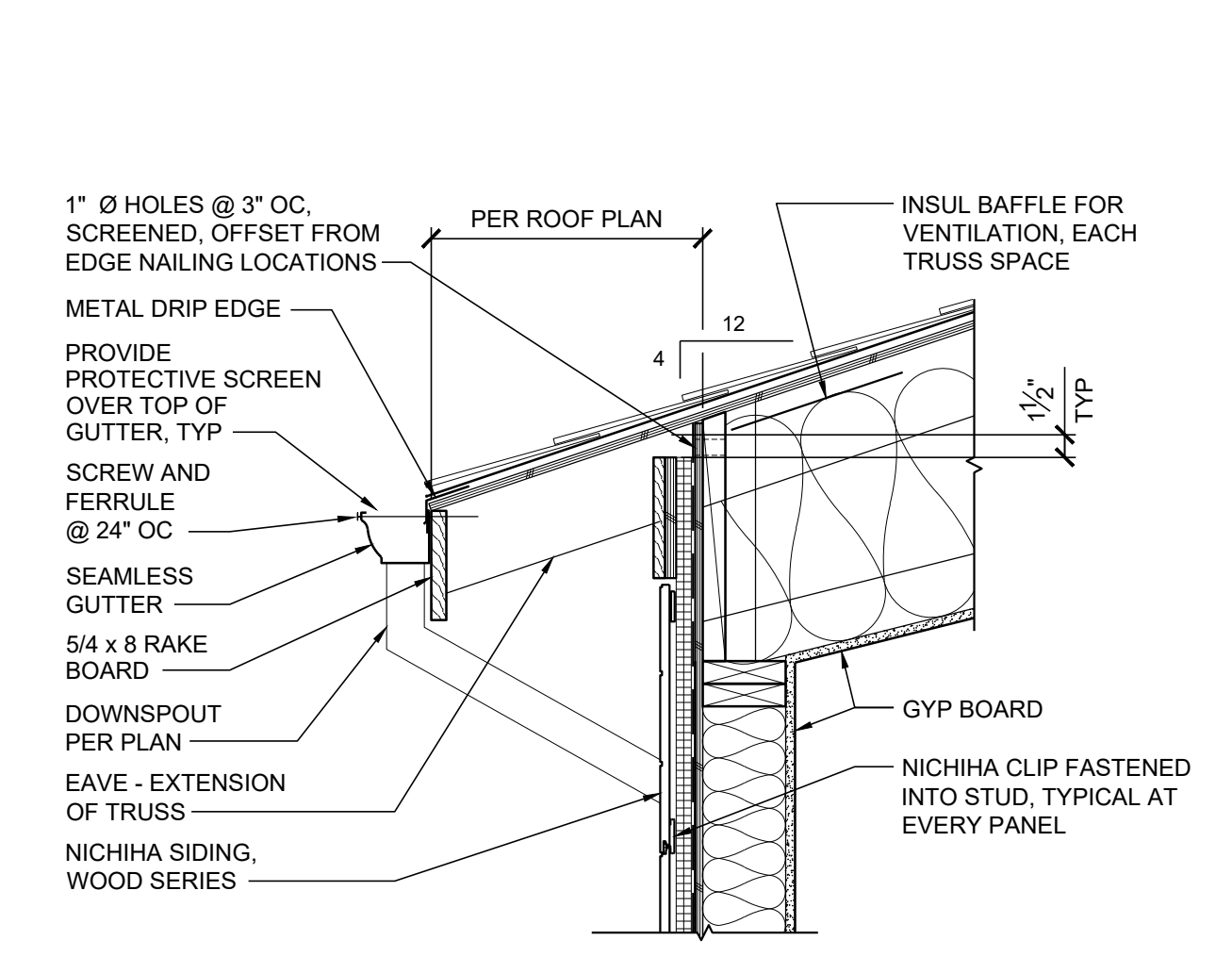
3 EAVE - SOUTH 1" = 1'-0"
