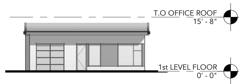
4 OFFICE - EAST ELEVATION SCALE: 1/16" = 1'-0"
