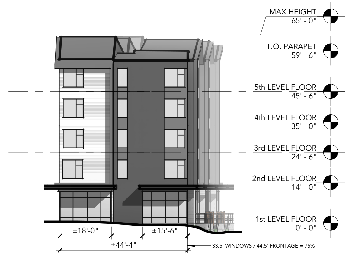
2 EAST ELEVATION SCALE: 1" = 20'-0"
