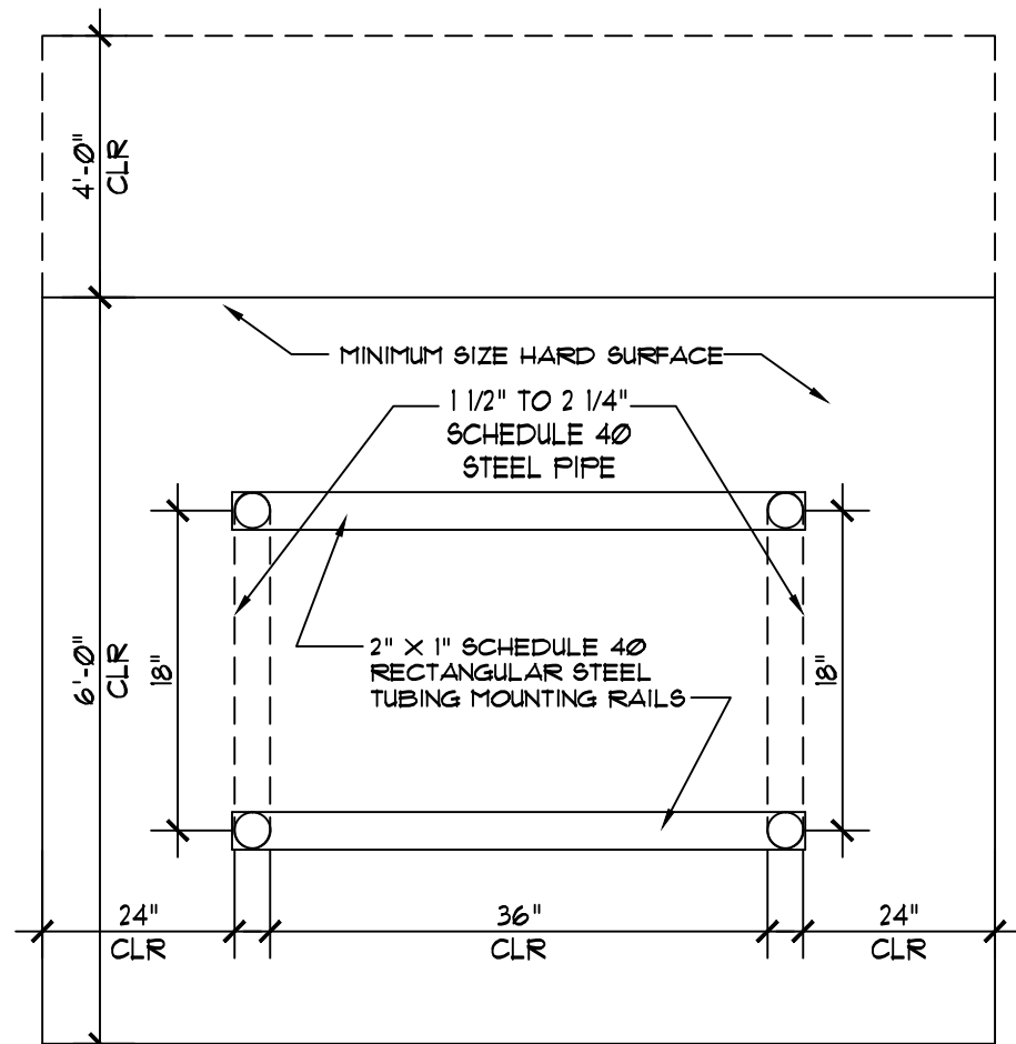
PLAN VIEW - MULTIPLE "U"
