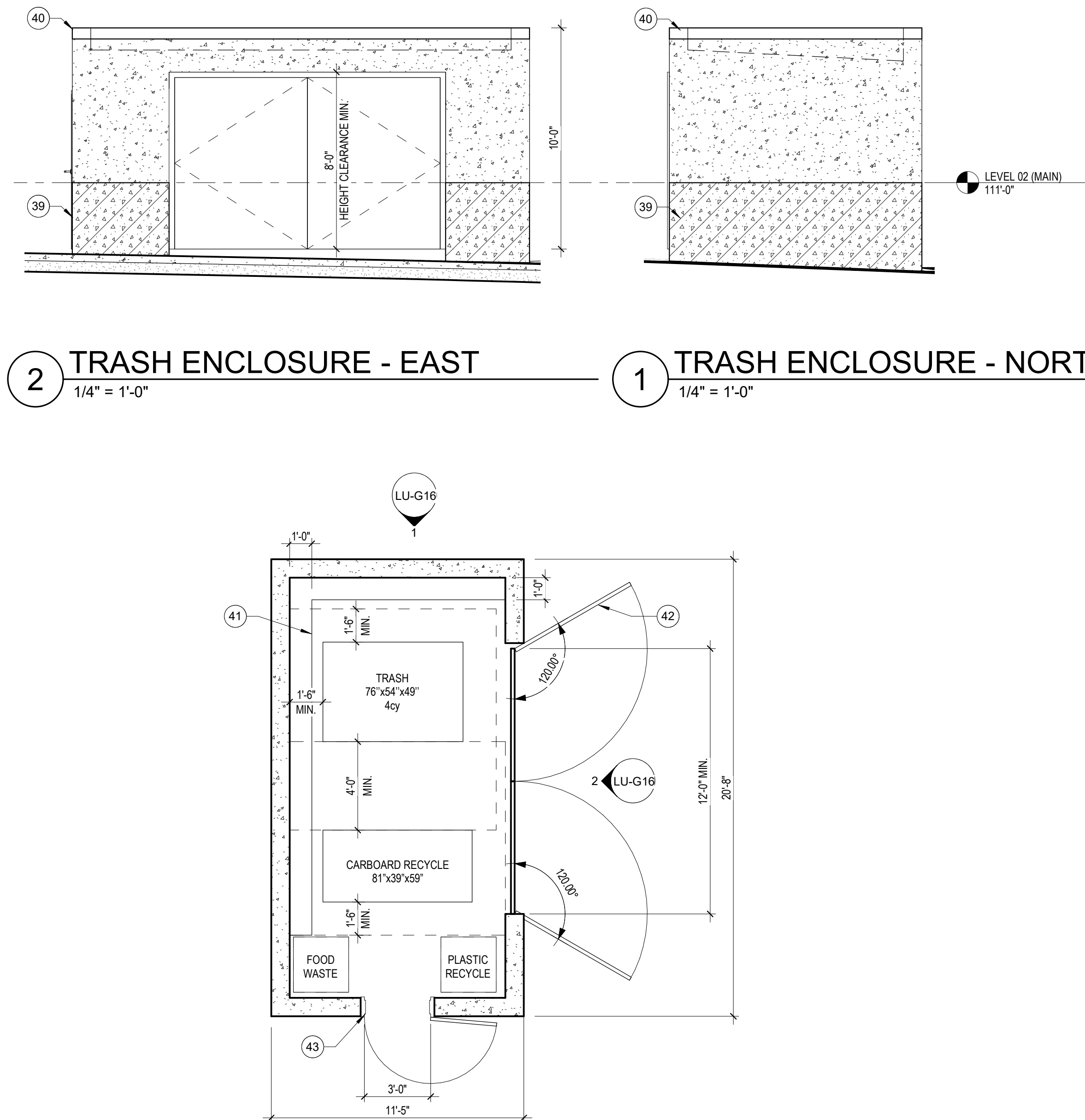
3 ENLARGED PLAN - TRASH ENCLOSURE 1/4" = 1'-0"
