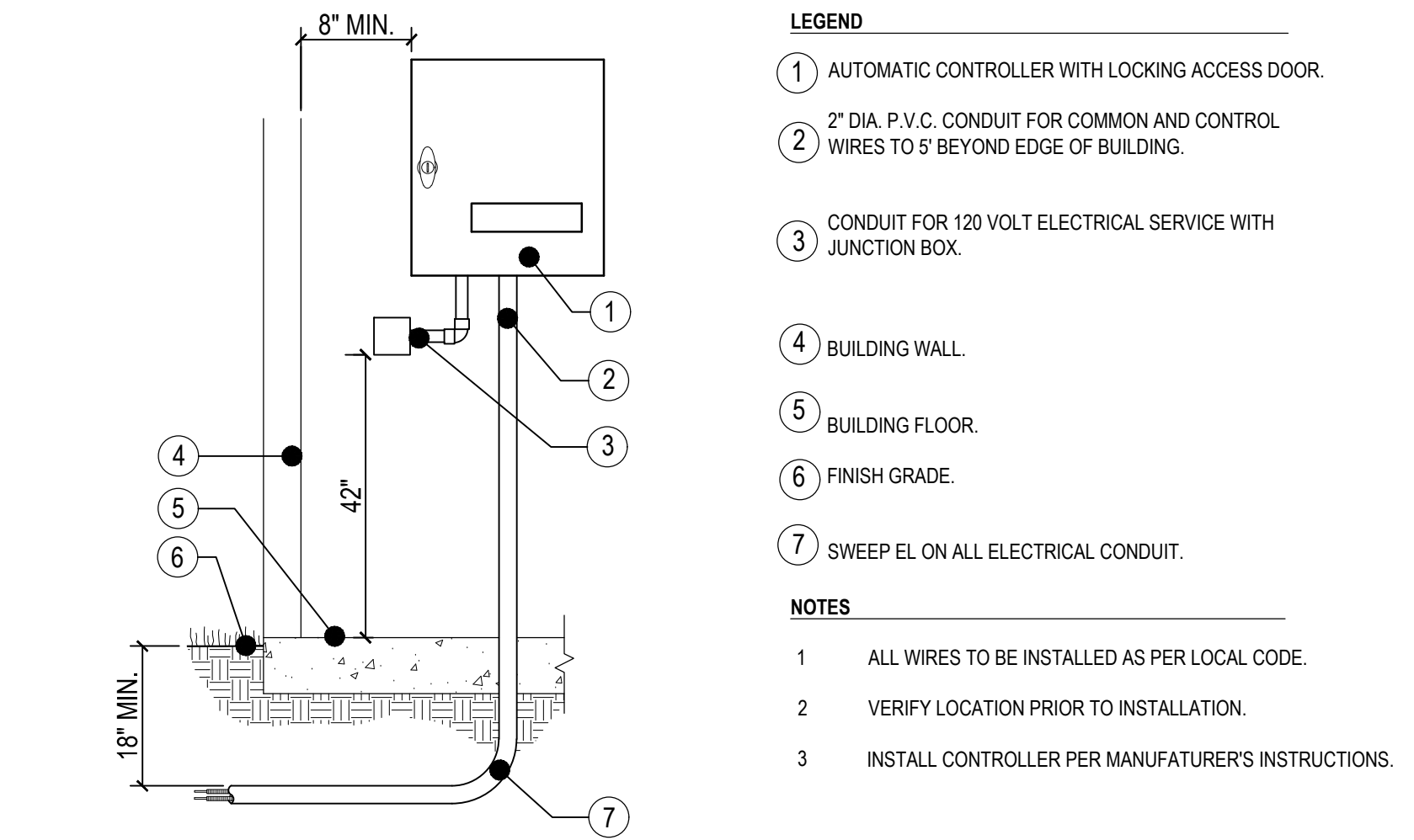
1 WALL MOUNTED CONTROLLER ## SCALE: NTS
