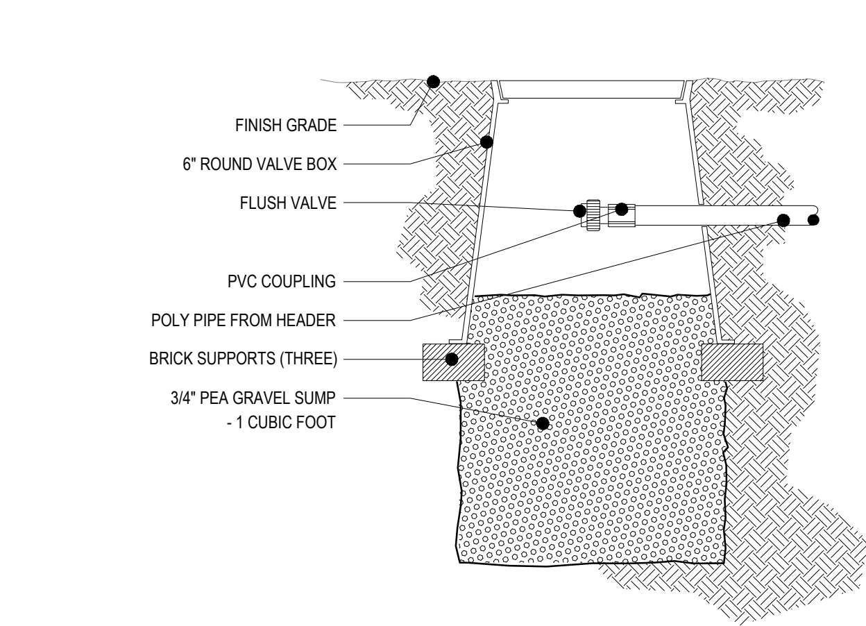
7 FLUSH VALVE ## SCALE: NTS
