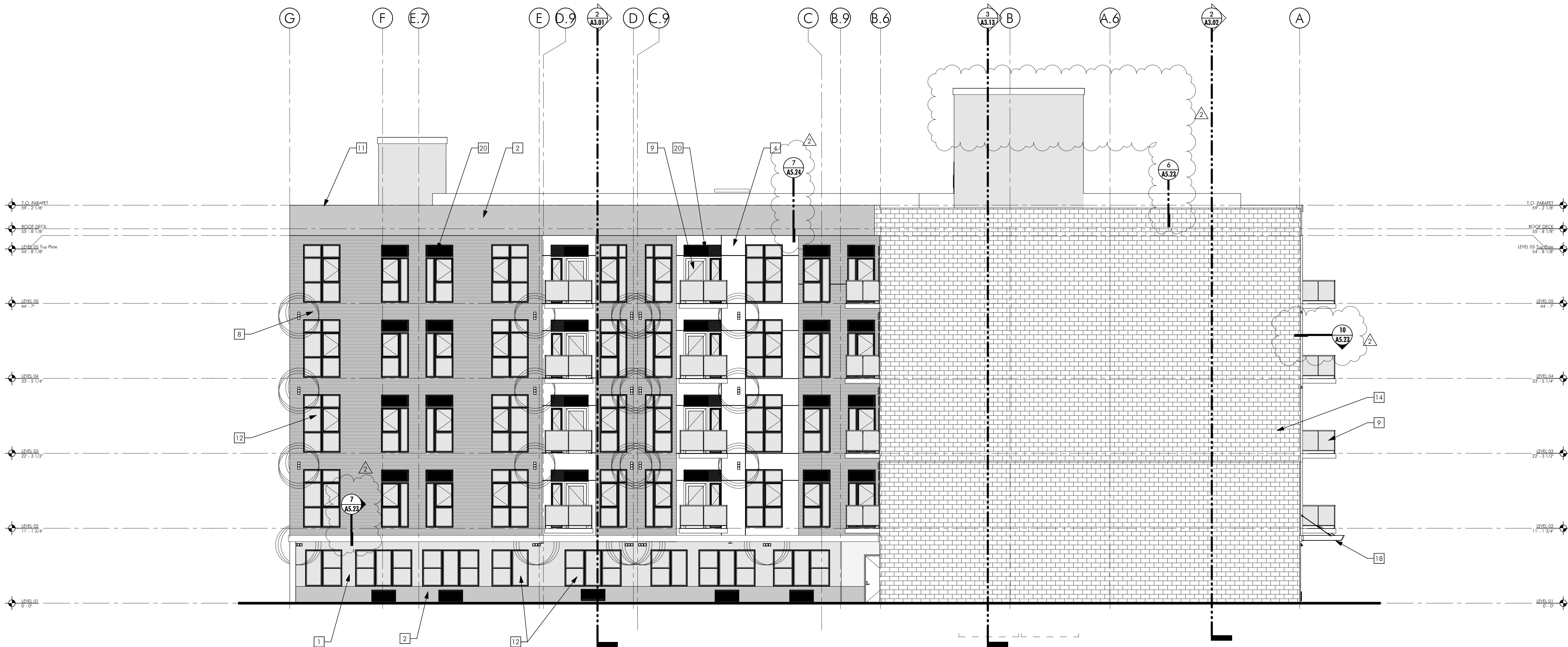
1 EAST ELEVATION
