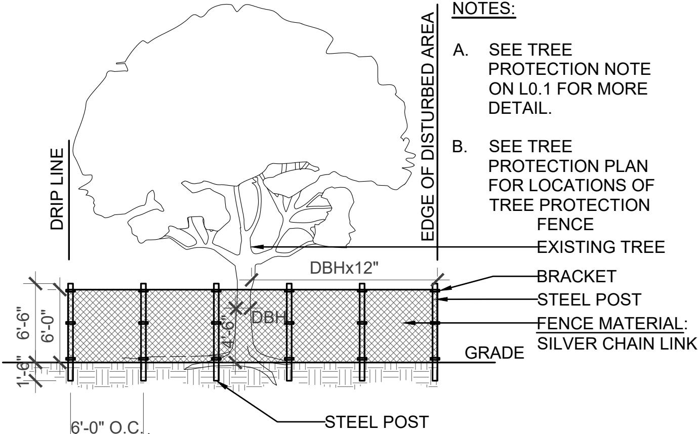
2 TREE PROTECTION FENCE SCALE: 1/8"= 1'-0"
