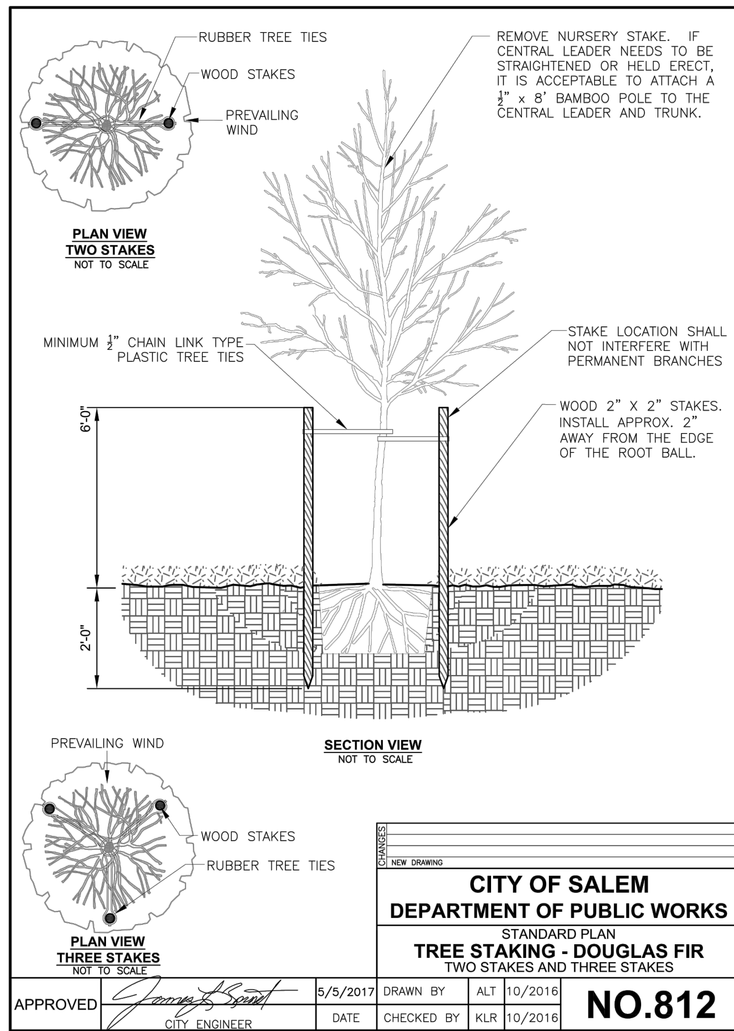
C4 TREE STAKING NO SCALE
