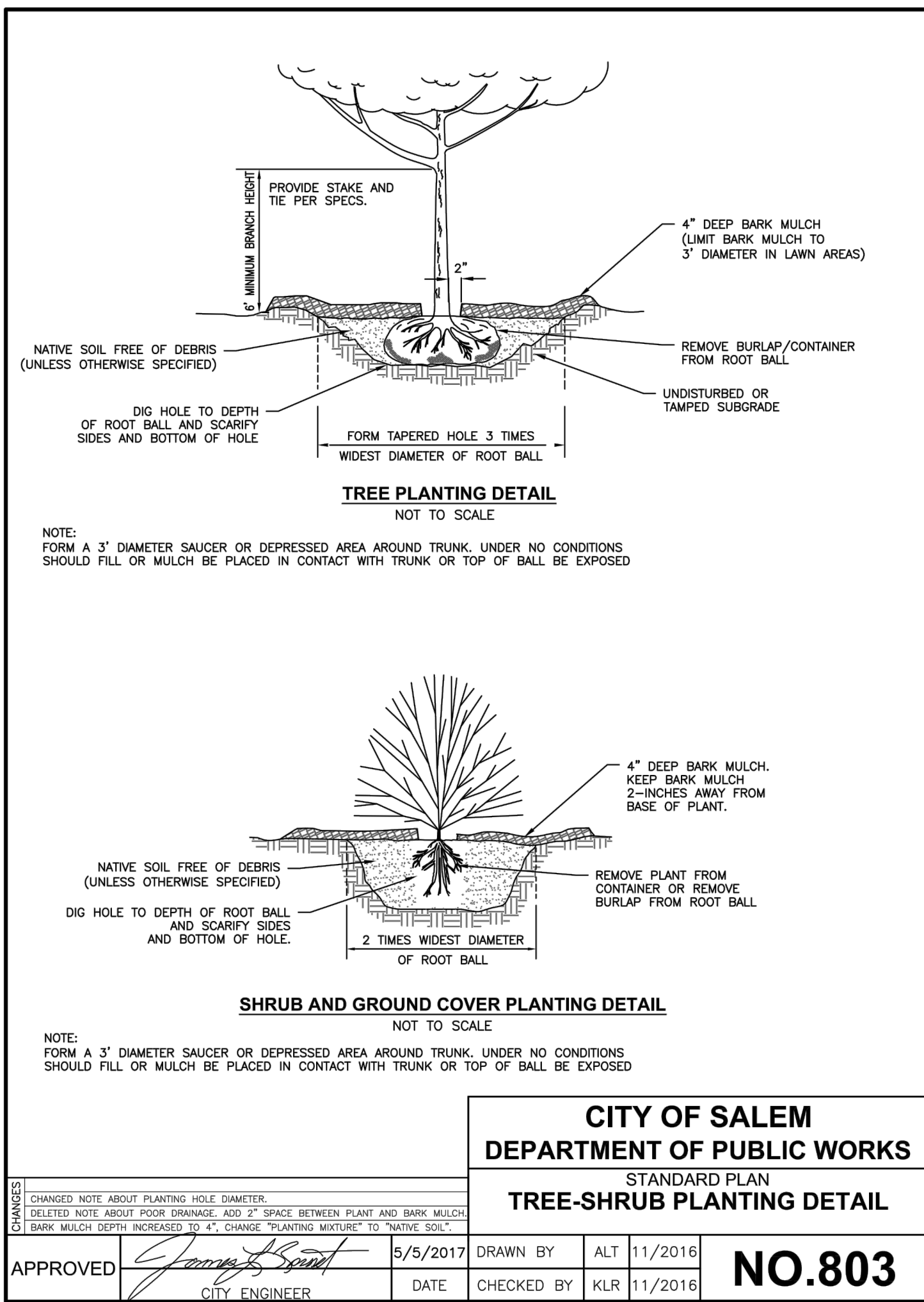
C1 TREE - SHRUB PLANTING NO SCALE
