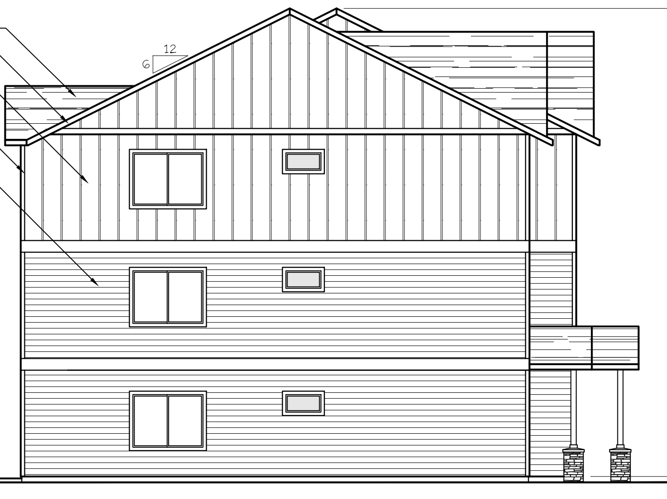
NORTH ELEVATION (TYPE A UNITS) SCALE: 1/8" = 1'-0" BLD. 3
