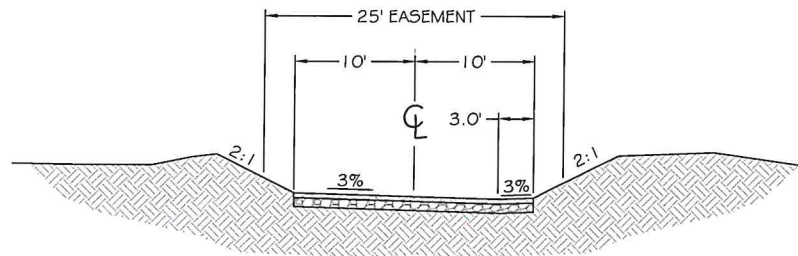
3 TYPICAL SECTION - FLAGLOT ENTRANCE SCALE: NTS
