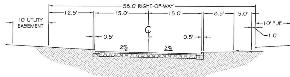
2 TYPICAL SECTION - FELTON ST STA 25+77-23+80 SCALE: NTS
