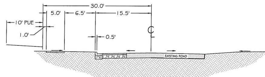
5 TYPICAL SECTION - SALEM HEIGHTS AVE SCALE: NTS
