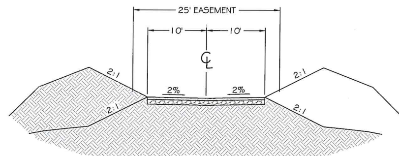
4 TYPICAL SECTION - FLAGLOT DRIVEWAY SCALE: NTS
