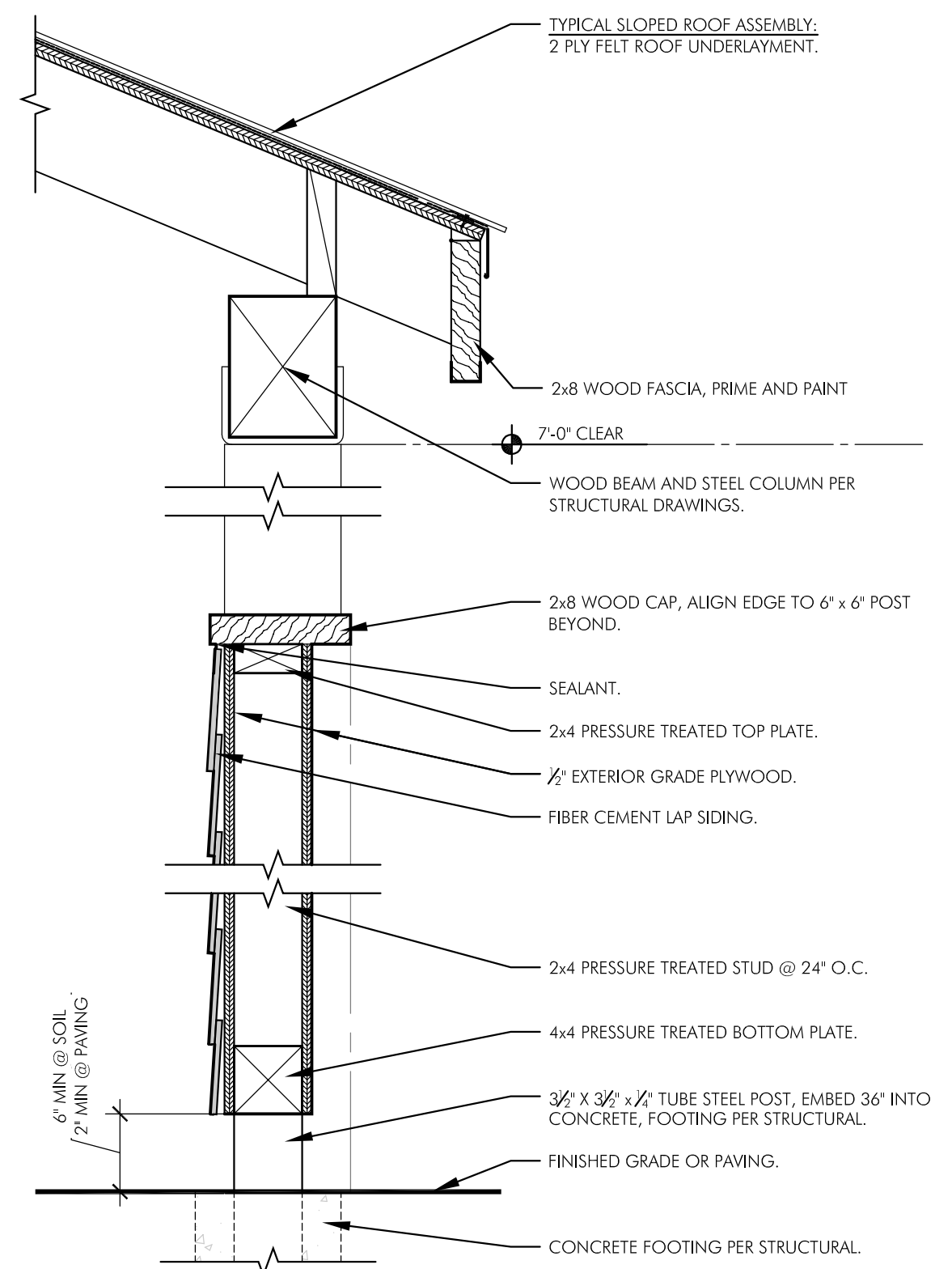
5 TRASH ENCLOSURE SECTION
