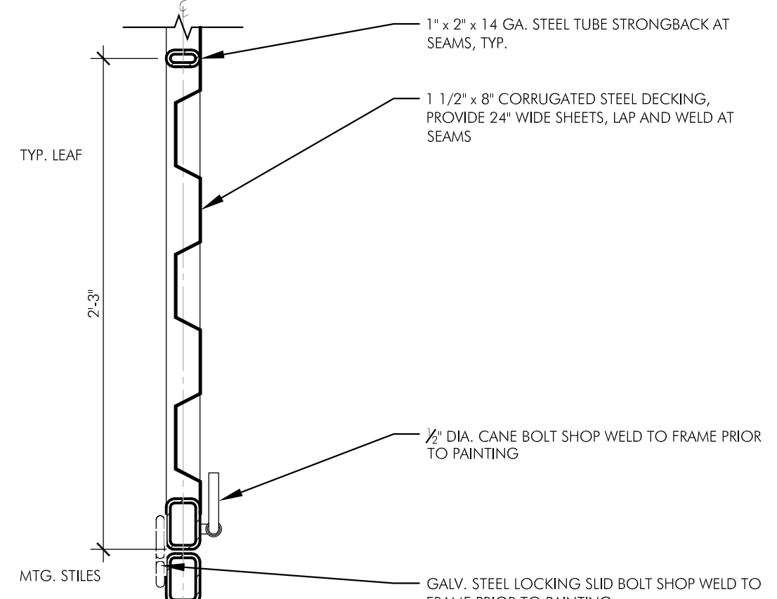
4 TRASH ENCLOSURE GATE DETAIL
