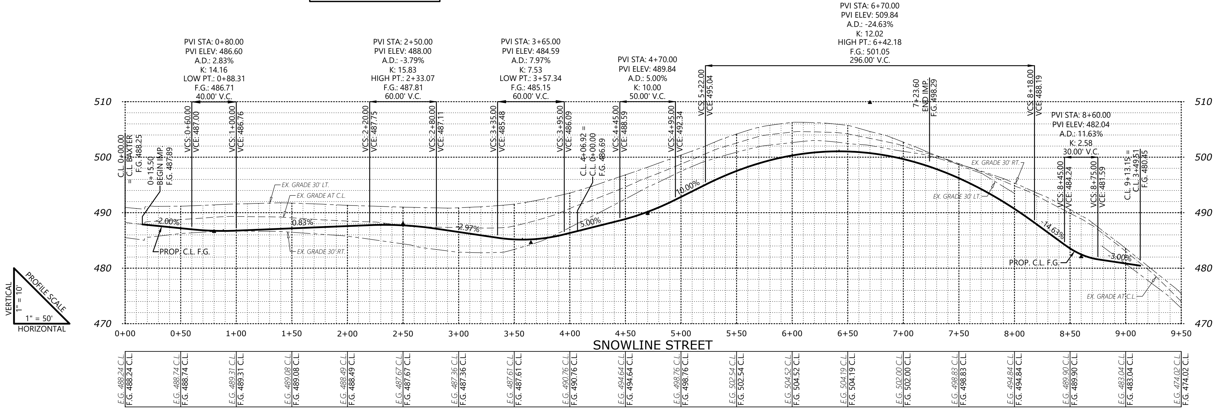
SEE SHEET 405 FOR STRUCTURAL STREET SECTION
