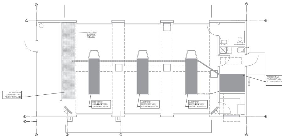
1 PLUMBING - SPILL CONTAINMENT PLAN 1/4"=1'-0"
