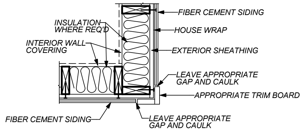
C A1 OUTSIDE WALL CORNER 1" = 1'-0"
