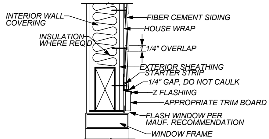
B A1 WINDOW/DOOR HEADER 1" = 1'-0"
