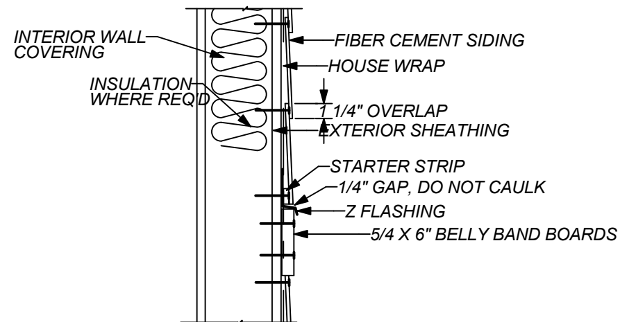
D A1 6" BELLY BAND 1" = 1'-0"
