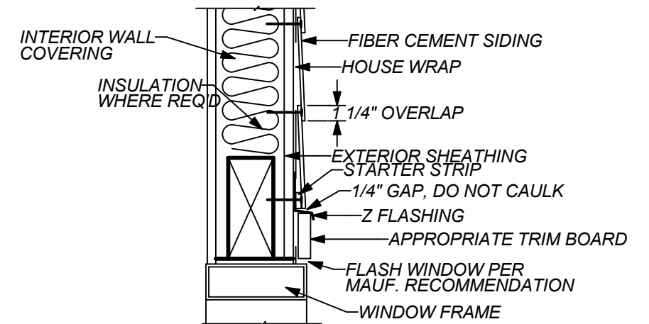
B A1 WINDOW/DOOR HEADER 1" = 1'-0"
