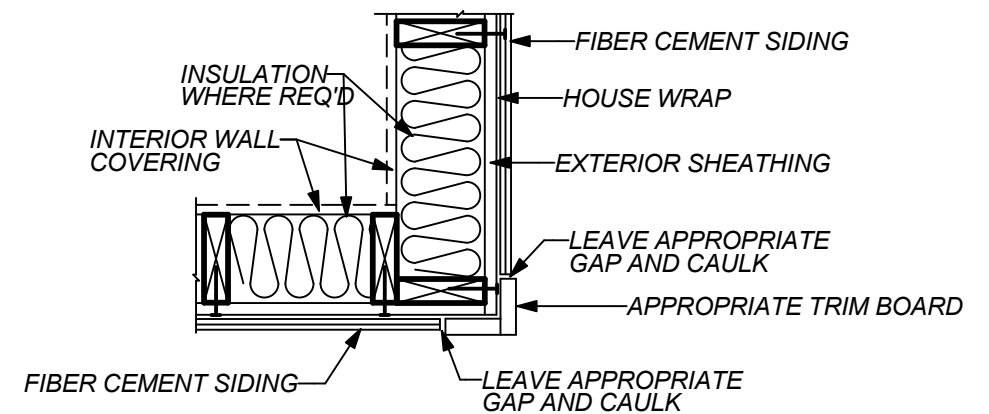
C A1 OUTSIDE WALL CORNER 1" = 1'-0"
