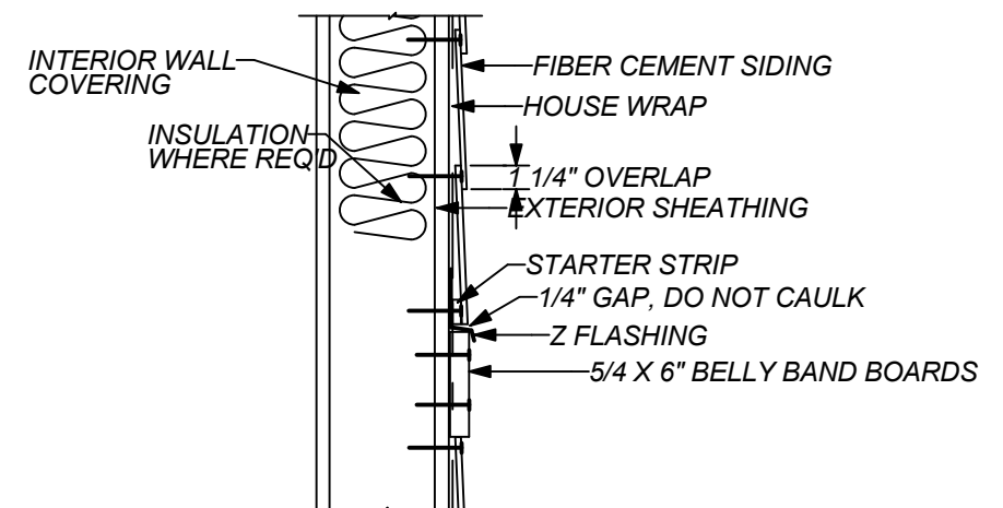
D A1 6" BELLY BAND 1" = 1'-0"
