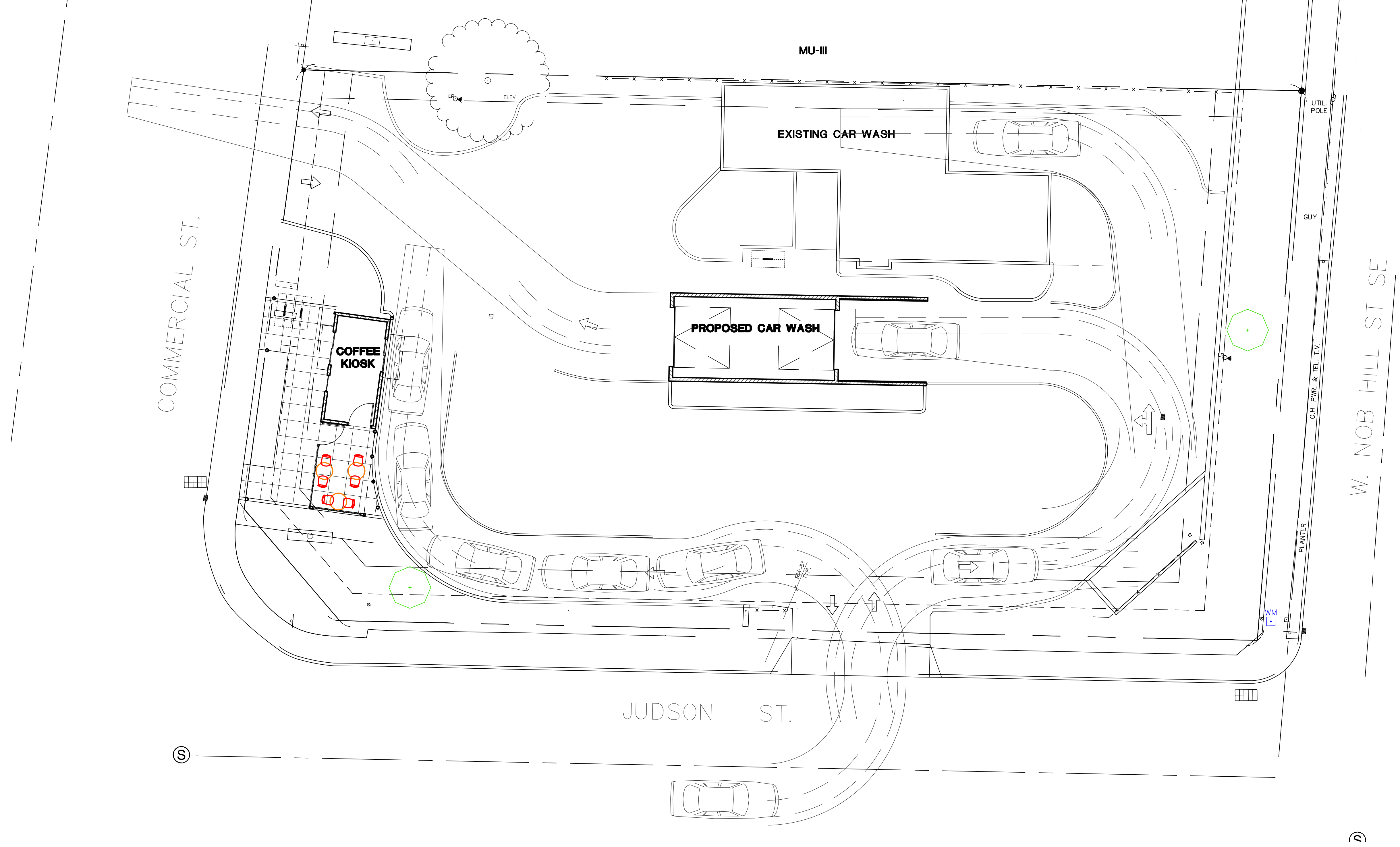
PROPOSED SITE CIRCULATION PLAN SCALE: 1" = 10' 0 5 10 20
