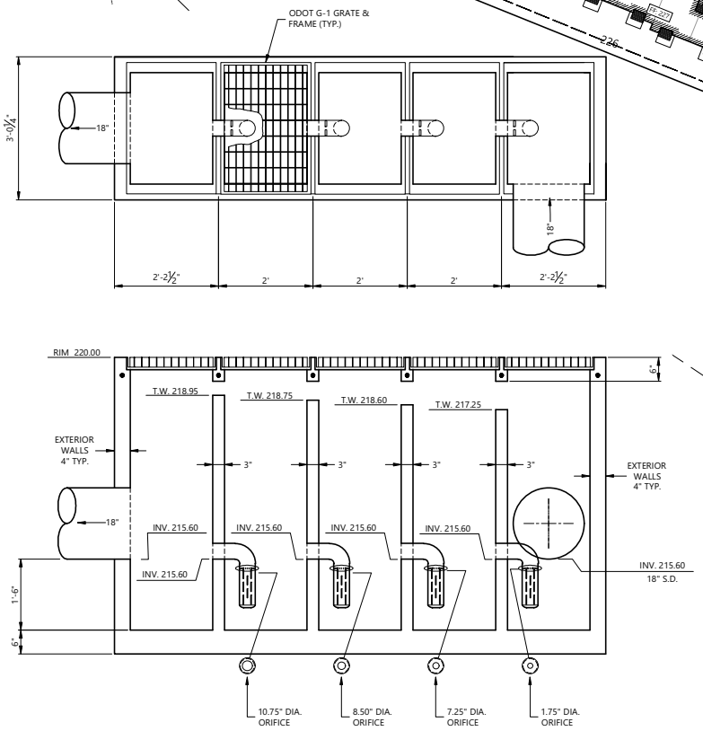
PRIVATE STORM WATER DETENTION CONTROL STRUCTURE NE
