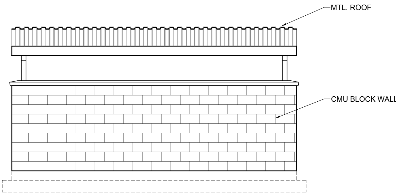
3 REAR ELEVATION A0.04 SCALE: 1/4" = 1'-0"
