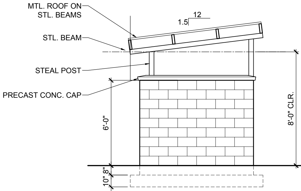
2 SIDE ELEVATION TYP. A0.04 SCALE: 1/4" = 1'-0"
