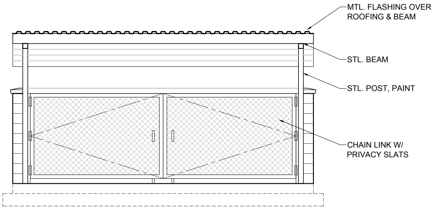
4 FRONT ELEVATION A0.04 SCALE: 1/4" = 1'-0"
