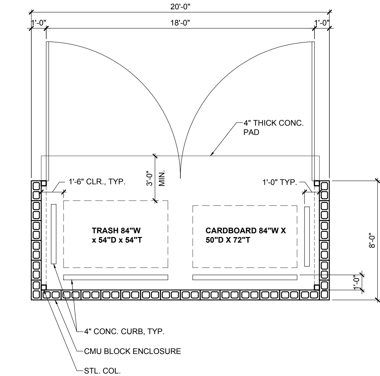
1 TRASH ENCLOSURE PLAN A0.04 SCALE: 1/4" = 1'-0"
